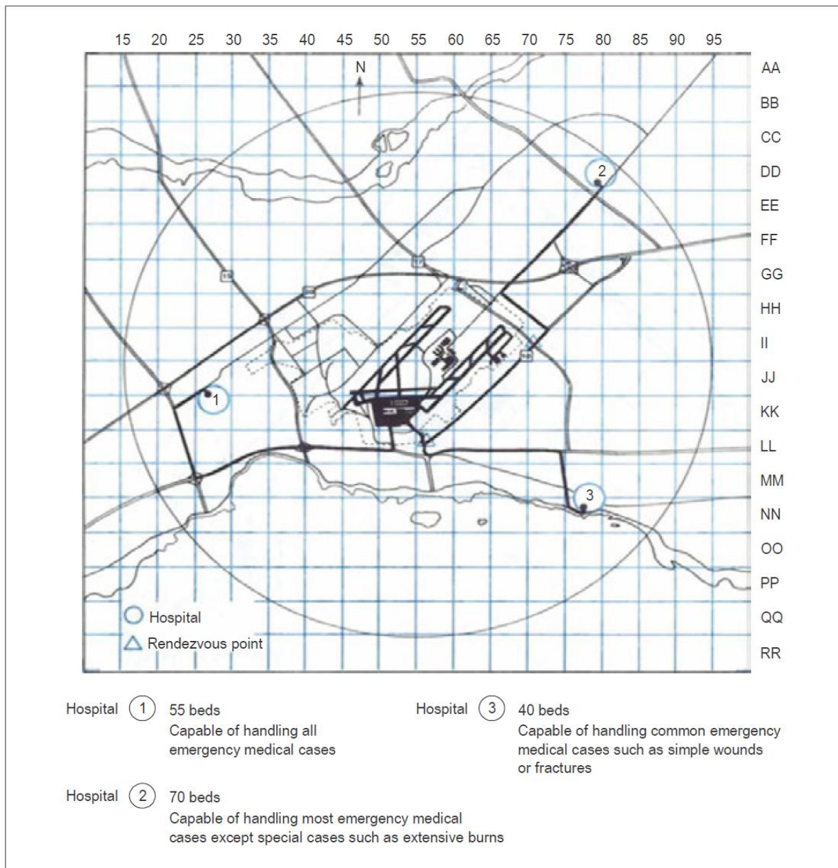
Figure 11-2. Sample grid map — airport and surrounding community
